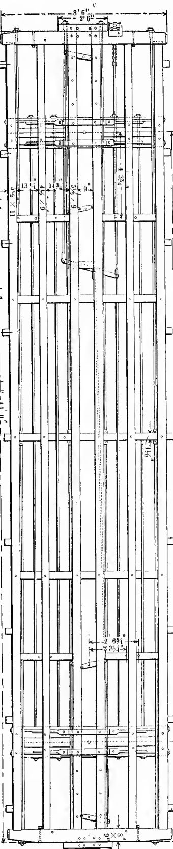
Fig. 293. Plan of Underframe. FLAT-CAR BODY, FOR LONG TIMBERS. ENSIGN MANUFACTURING COMPANY. Length, 41 ft. Capacity, 60,000 lbs. Weight, 23,700 lbs. Inverted King and Queen Post Trussing, with Counterstruts to prevent Buckling. (General view is shown in Fig. 19.)
